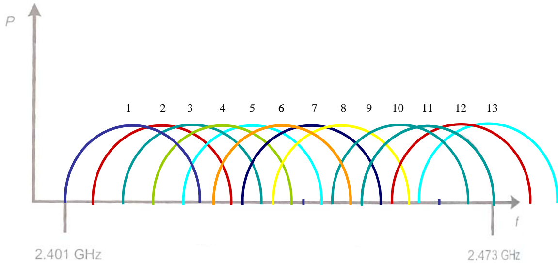
Figure 2. 802.11b Direct Sequence Channels
