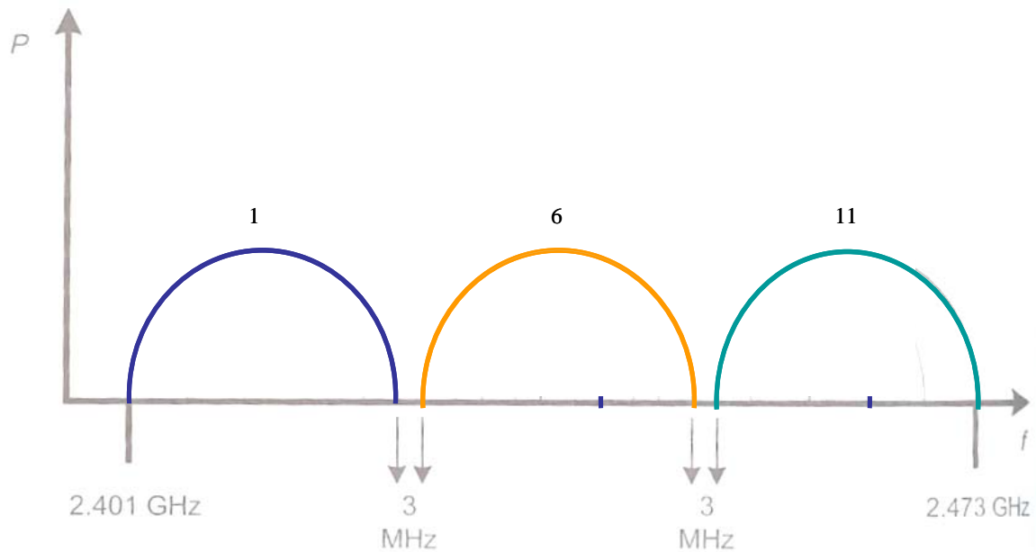
Figure 3. Non-overlapping 802.11b Channels
