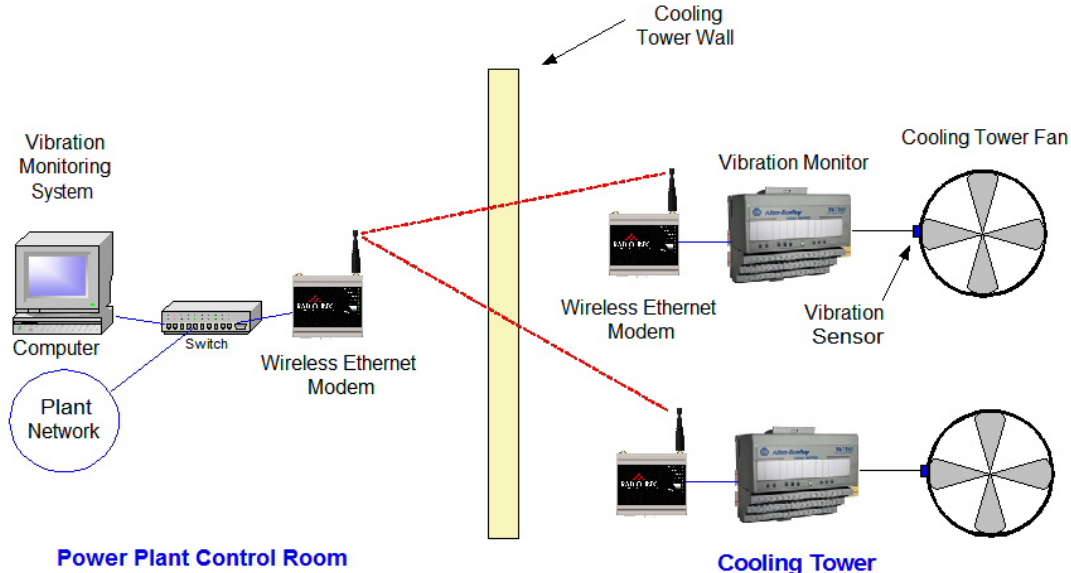
Figure 5. Wireless Cooling Tower Application
